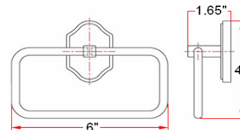
towel ring
