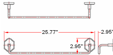
24" towel bar
