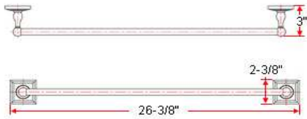
24" towel bar
