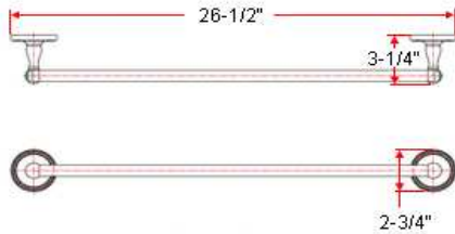
24" towel bar
