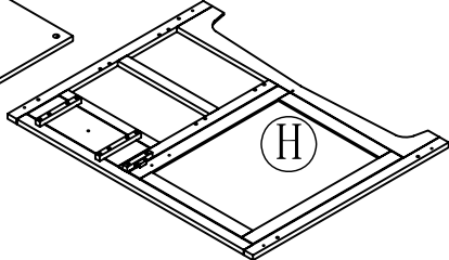
FRONT FRAME 1PC
